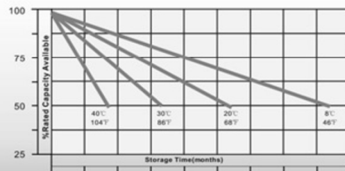
Self-Discharge at Different Temperatures
